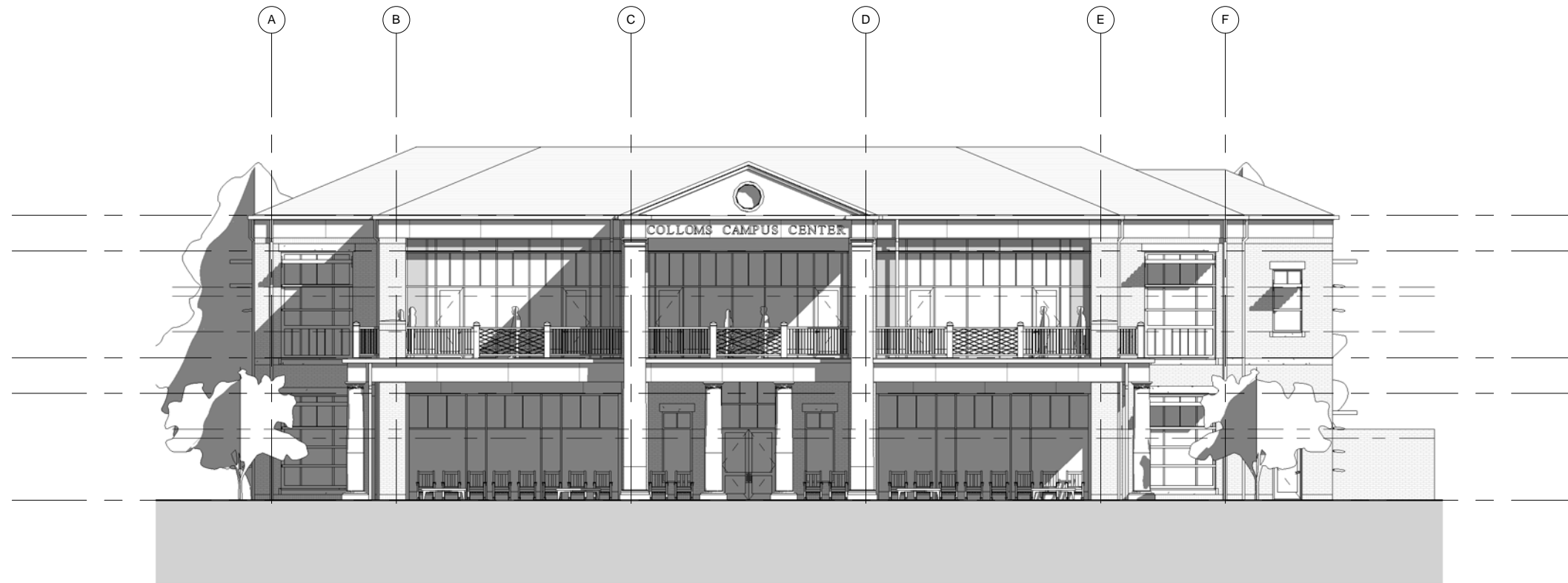
North Elevation
