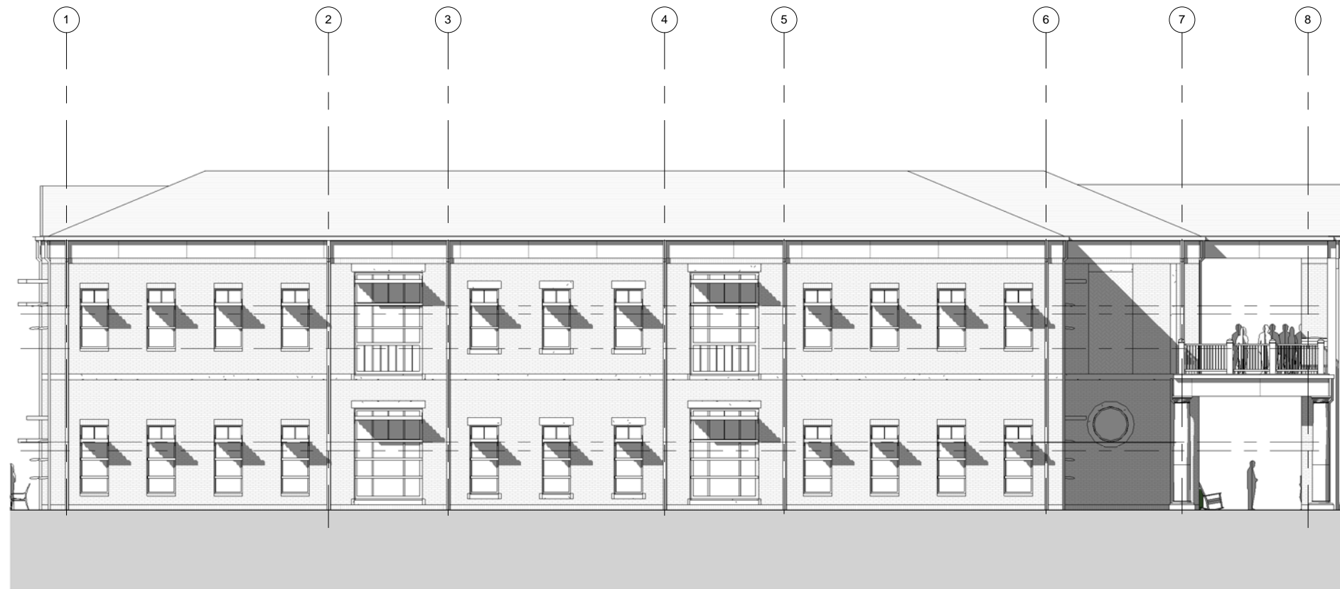
East Elevation
